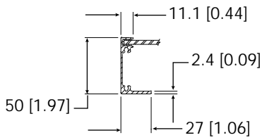
Section X-X
