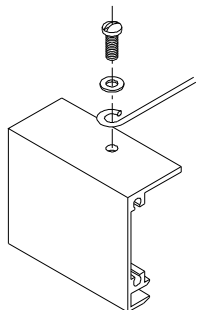
Grounding Detail
